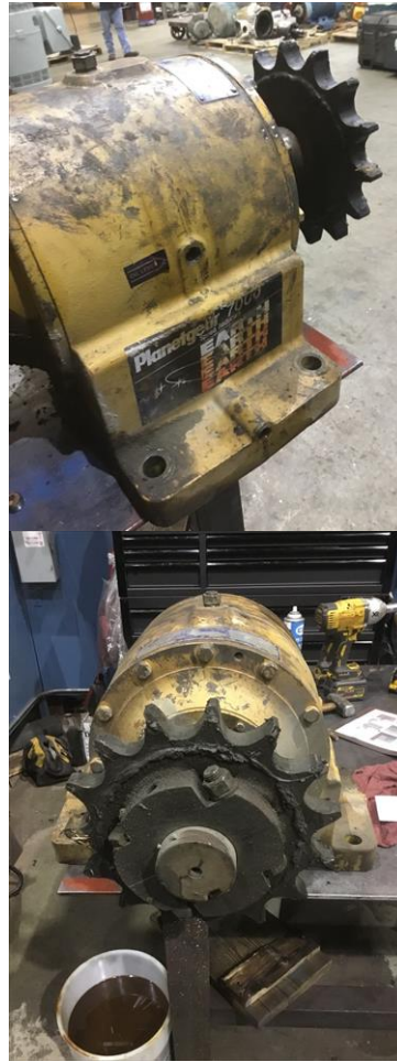
Shaft out 1 1/8
