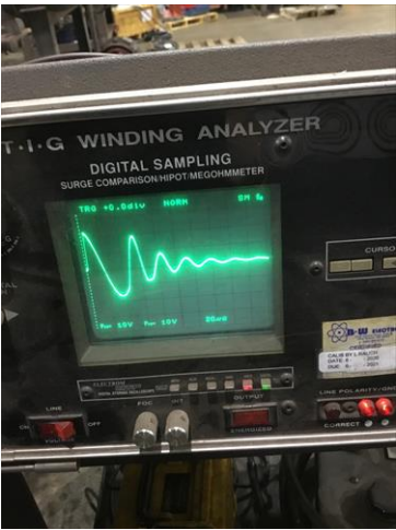
Armature test good
