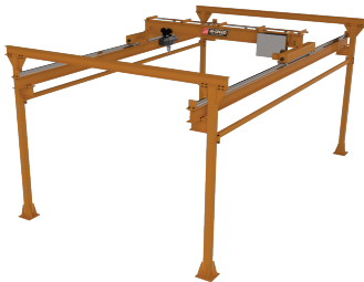
Model 811/813/491/492 Freestanding I-Beam Bridge Crane Workstations Capacities up to 15 Ton Manual or Motorized Freestanding Systems Ceiling Hung Systems Underhung or Top Running Turnkey Solutions Fully Customizable
