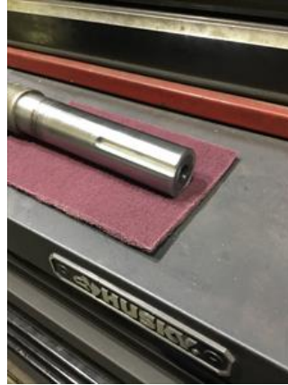
Welded and remachined input shaft. Finish dia. 1.7503 3/8" keyway 3" long
