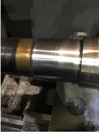
Welded and machined output shaft seal surface Dia. After machining 5.2513
