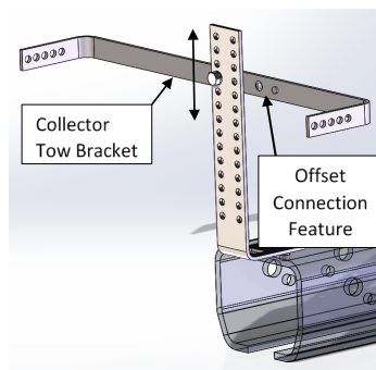
Diagram 10Q. Tow bracket directly mounted to mast.
