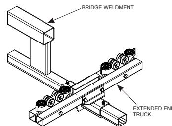
Diagram 5H. Installing extended clamping end truck. See TIP .
