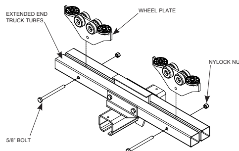
Diagram 5G. Installing wheel plates.
