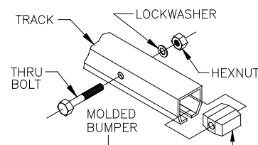
Diagram 5L. Installing end stop.
