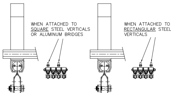
Diagram 10V. Bridge studs.
