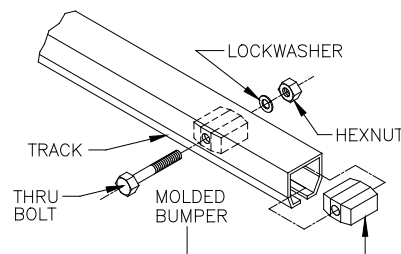
Diagram 8E. Installing end stops in bridge.
