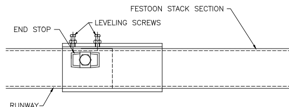
Diagram 7A. Installing festoon stack section.
