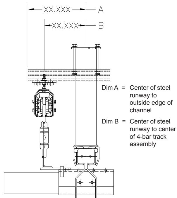
Diagram 10A. Runway A-B dimensions.
