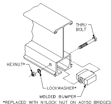
Diagram 5M. Installing end stop.
