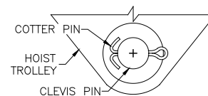
Diagram 5E. Installing cotter pin through trolley saddle clevis pin.
