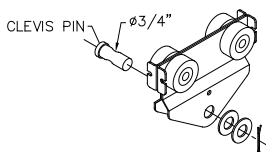
Diagram 5B. 250 series hoist trolley. Diagram 5C. 500 series hoist trolley. Diagram 5D. 1000, 2000 series hoist trolley.
