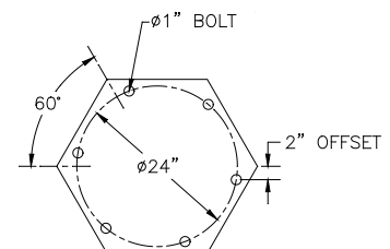
Diagram 3G. 6 bolt base bolt pattern.
