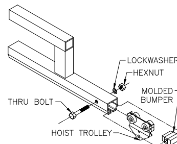
Diagram 5G. Installing hoist trolley and endstop.
