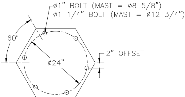
Diagram 3C. 6 bolt base bolt pattern.
