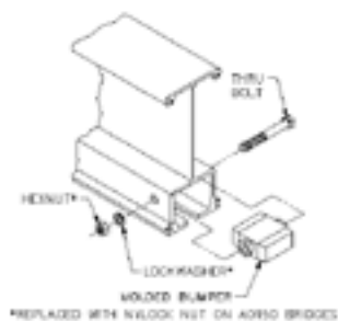
Diagram 4E. Installing standard endstop.
