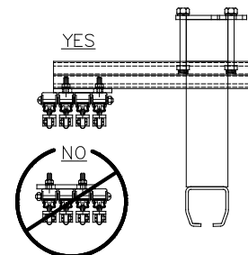
Diagram 10S. Conductix installation orientation.
