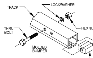
Diagram 11D. Installing endstop.
