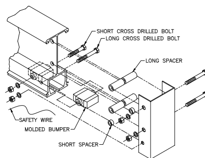
Diagram 4F. Installing the automotive style double wired endstop with endcap.
