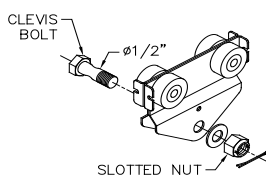
Diagram 6A. Installing hoist on 150#-250# hoist trolley.
