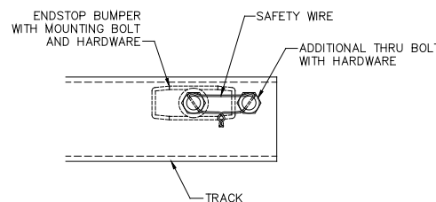
Diagram 11E. Double wired end stop.
