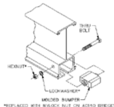
Diagram 5H. Installing end stop.
