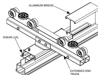
Diagram 5G. Installing extended clamping end truck. See TIP .
