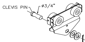
Diagram 6B. Installing hoist on 500# hoist trolley.
