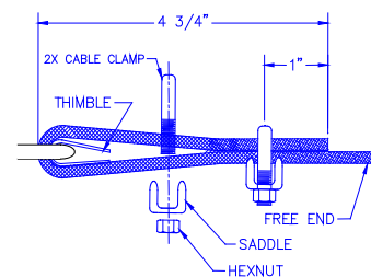
Diagram 11A. Saddling the cable on one end.
