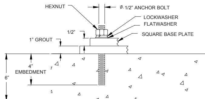
Diagram 2A. Typical square base plate anchor bolt embedment.
