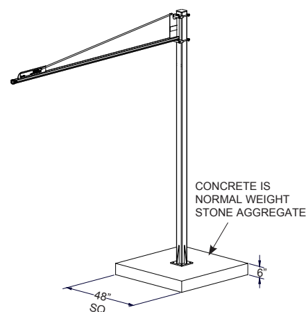
Diagram 2B. Foundation Requirements.
