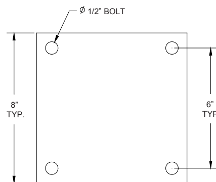
Diagram 2C. Square base plate pattern.
