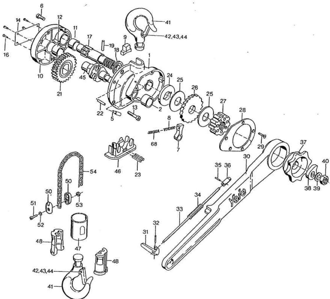
Parts for Model C 85 with roller chain
