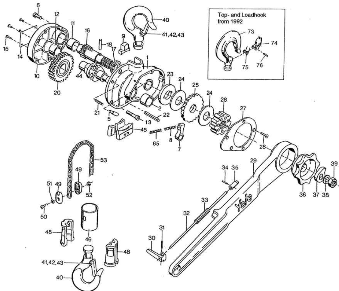
Parts for Model C 85 with roller chain
