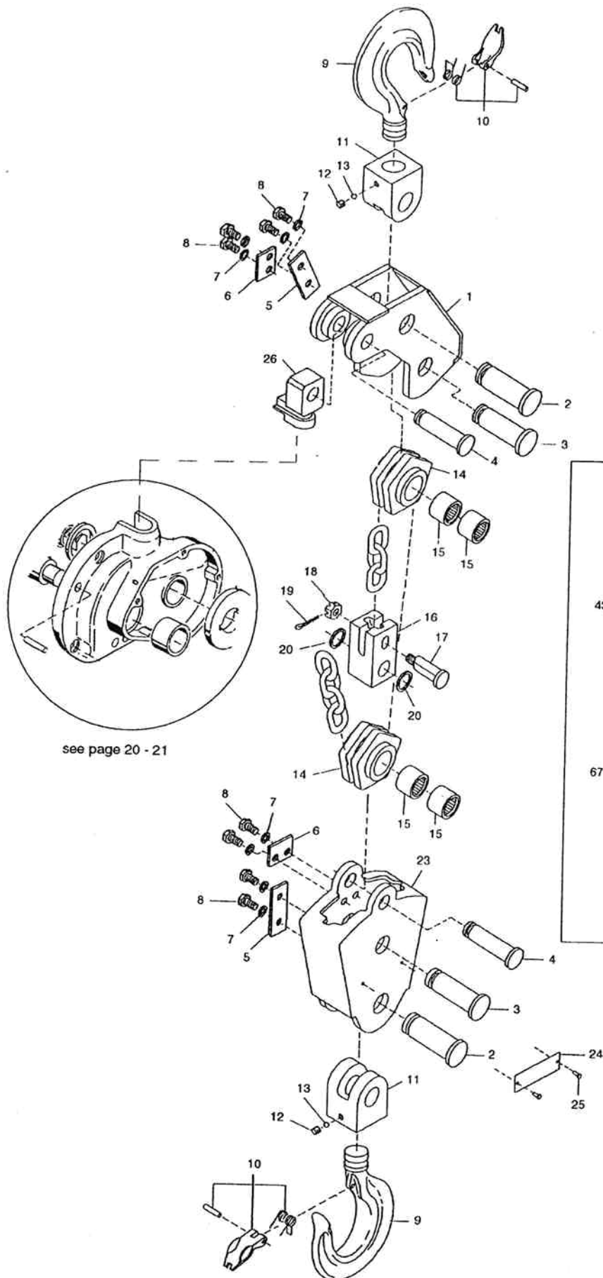
Parts for Model C85 with Roller Chain only
