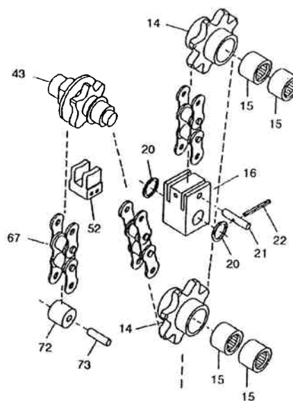
Parts for Model C85 with Roller Chain only
