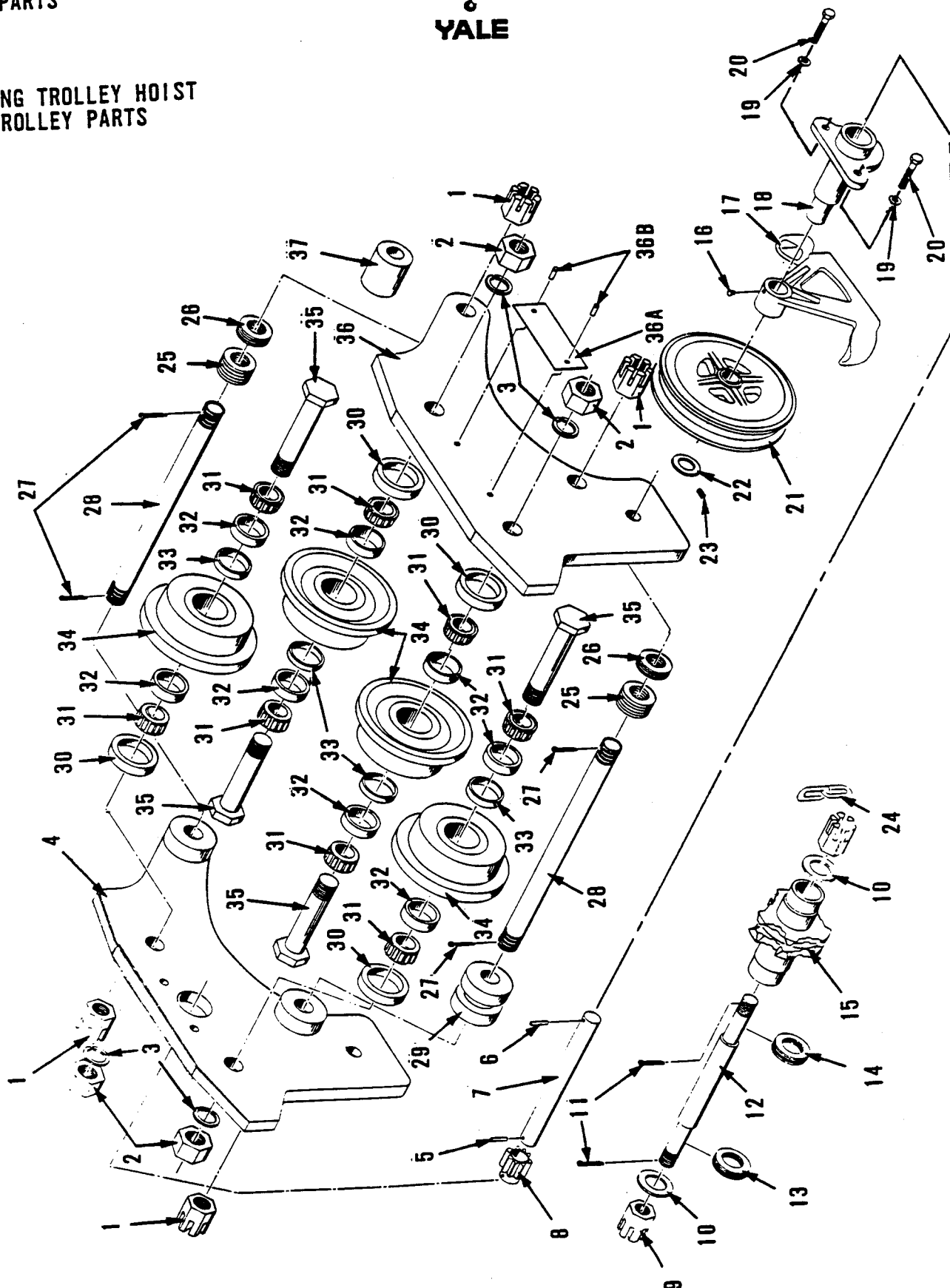
FIGURE 13. 8 TON LOAD KING TROLLEY HOIST, TROLLEY PARTS
