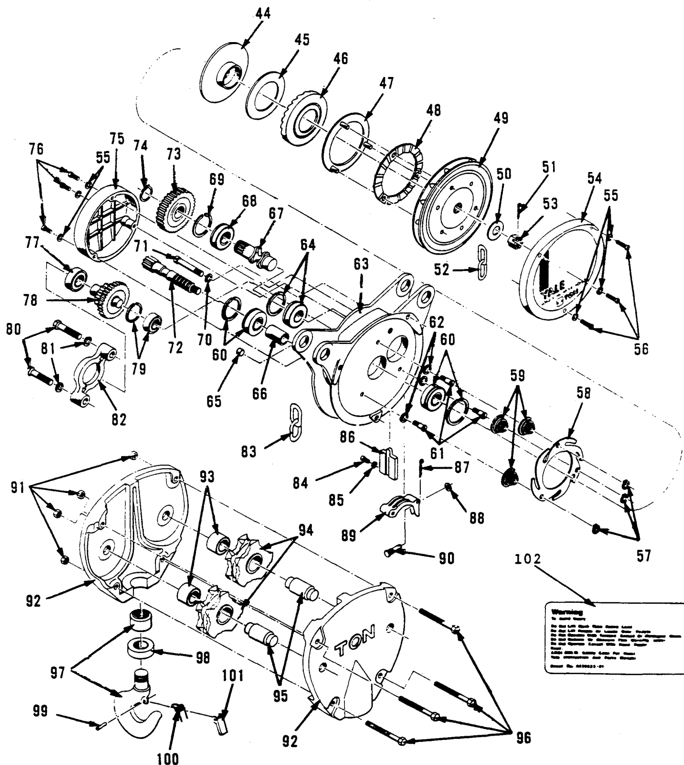
FIGURE 18. 12 TON LOAD KING TROLLEY HOIST. HOIST PARTS
