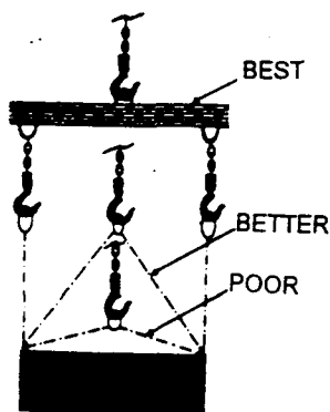
CONSIDER THESE ANGLES WHEN LIFTING LOAD
