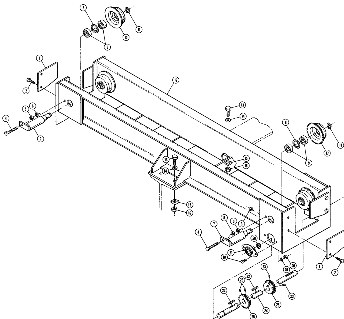
Figure 8. Geared Truck. Catalog Numbers 905369 and 905525. (Only 1 Truck Shown)
