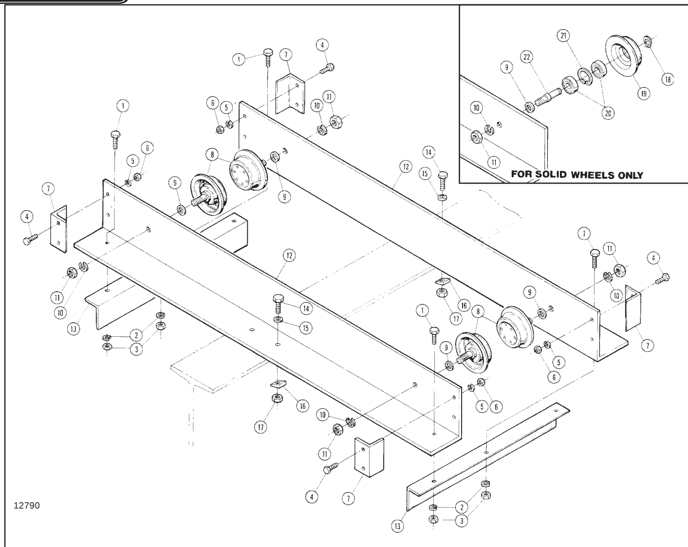
Figure 3. Truck Parts
