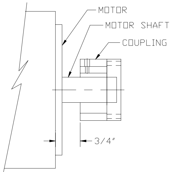
Figure 2. Coupling Location.
