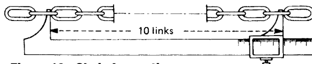
Figure 10 - Chain Inspection
