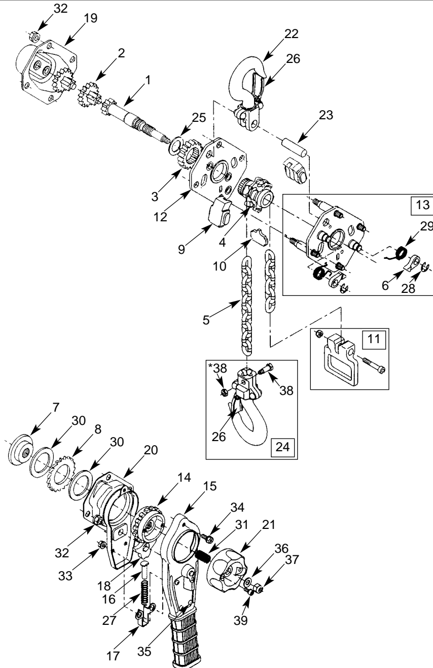
Figure 15 - .75 & 1.5 Ton Models
