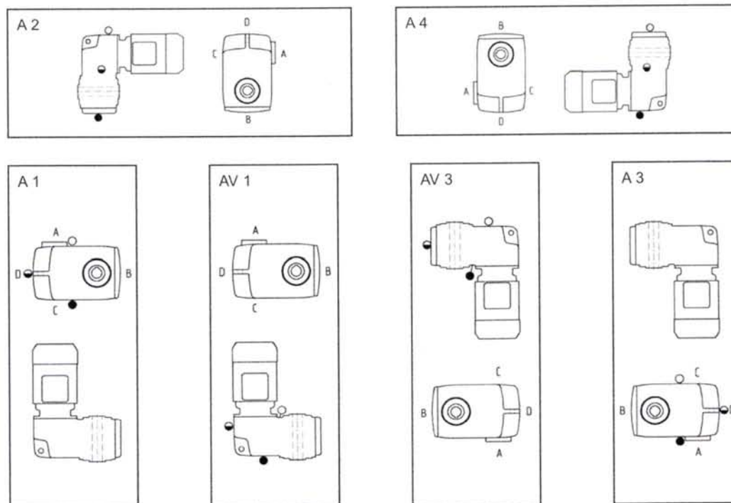
Image 11 : Constructions of flat gear motors
