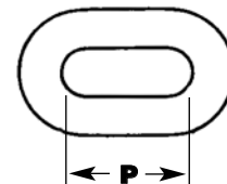
Figure 1 - Chain Wear Measurement
