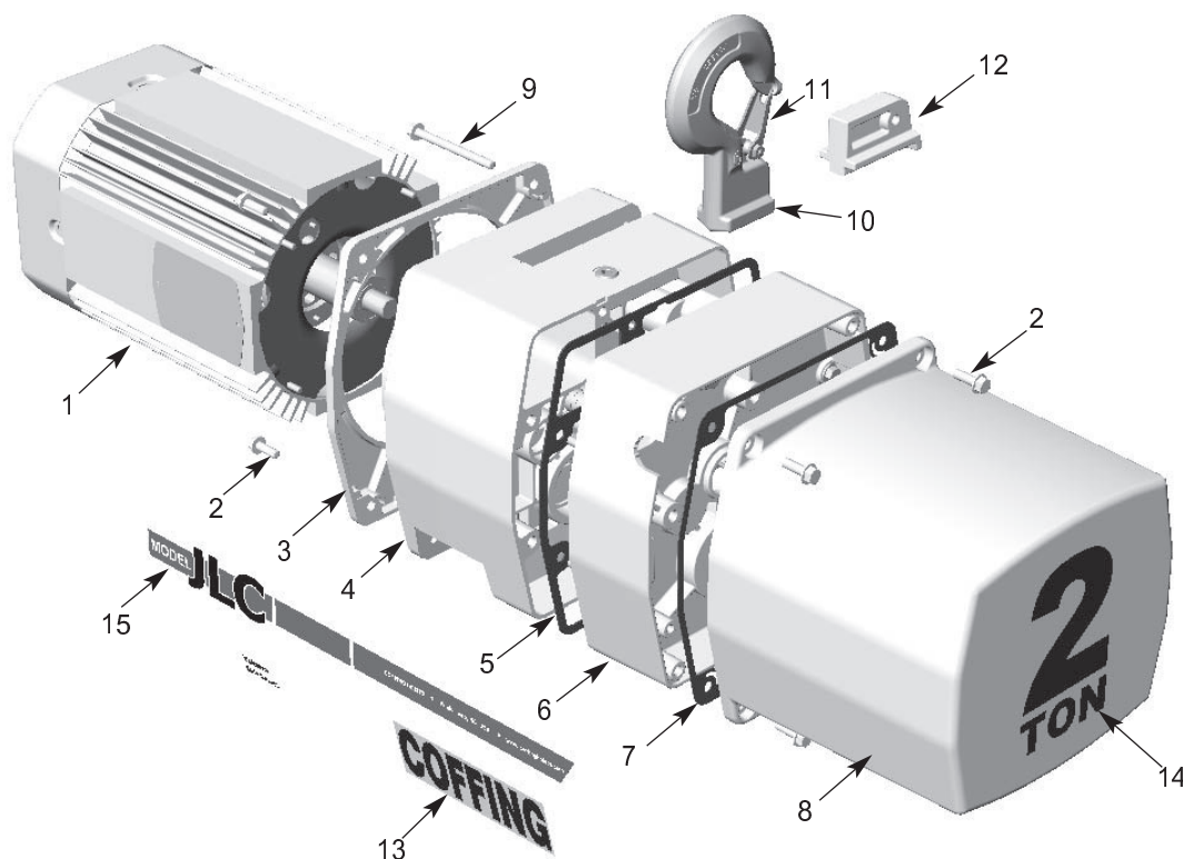
Figure 12 - Basic Hoist
