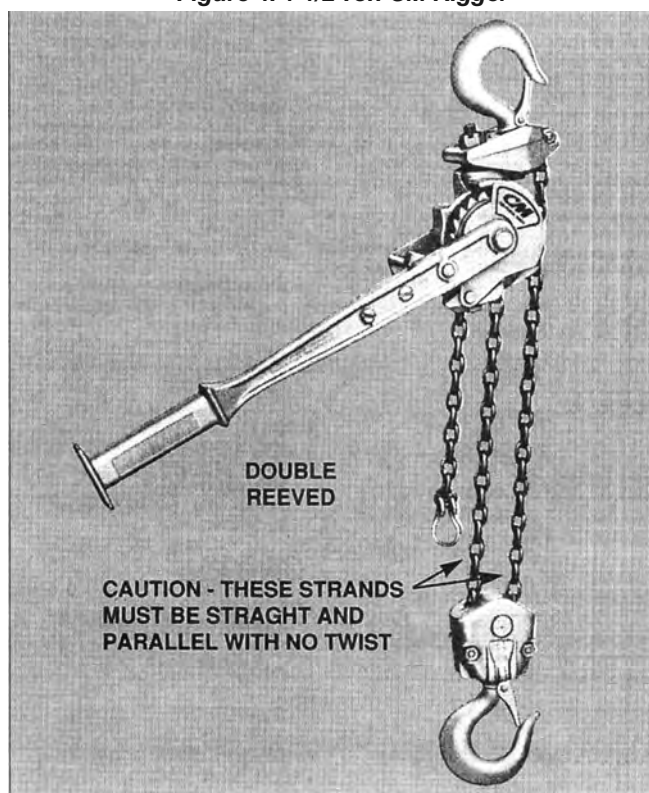
Figure 4. 1 1/2 Ton CM Rigger
