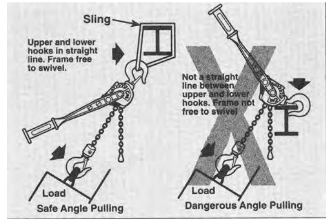
Figure 1. Angle Pulling
