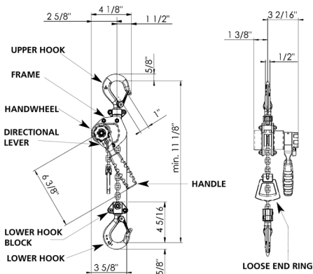
SERIES 603 LEVER HOIST
