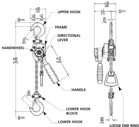
FIGURE 1 SERIES 602 LEVER HOIST
