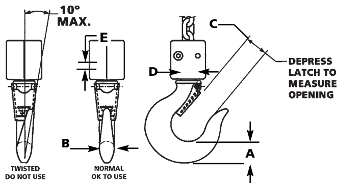
Figure 3 - Hook Inspection
