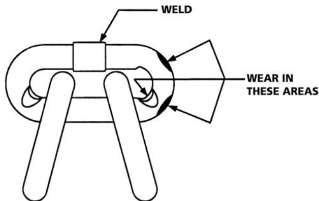
Figure 4 - Chain Inspection
