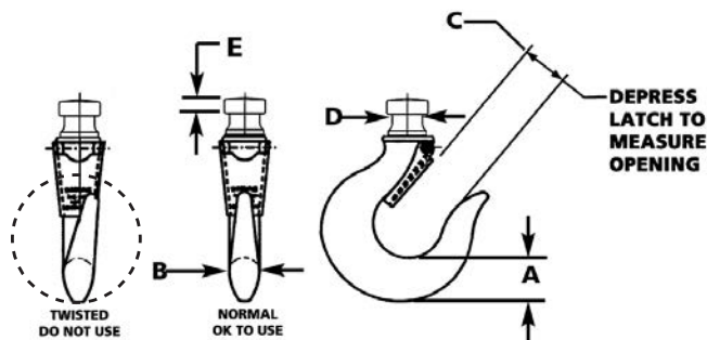
Figure 3 – Hook Inspection
