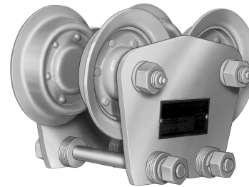
1 Ton Rated Load Push Type Trolley
