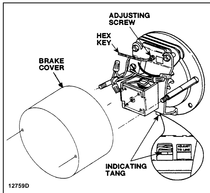
Figure 1. Hoist Motor Brake
