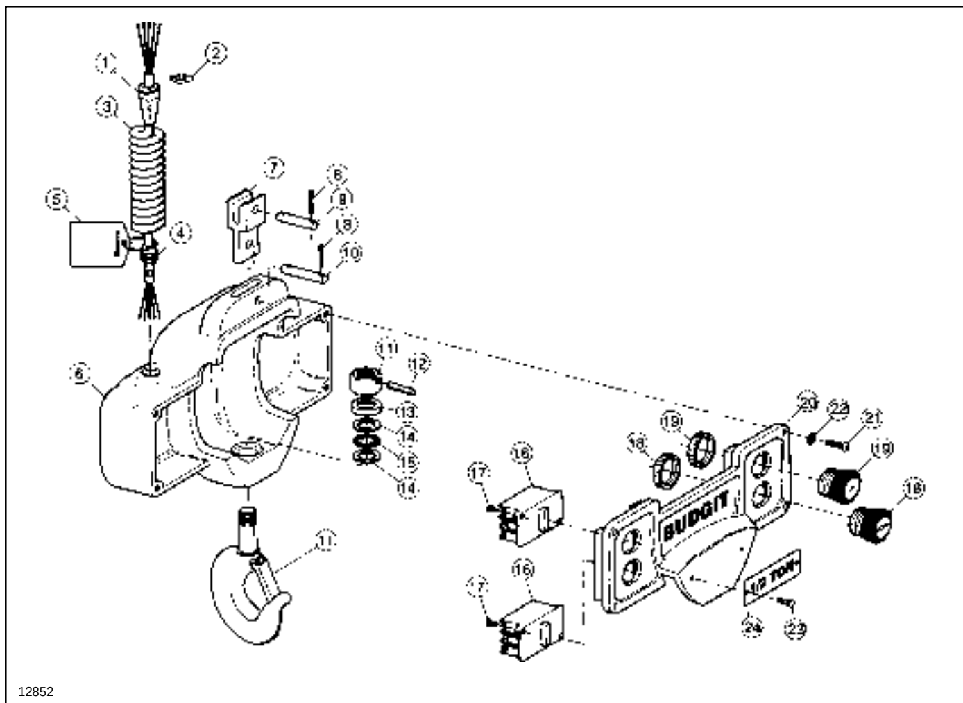
Figure 1. Loadpoint Control.
