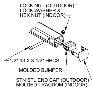
Diagram 5E. Installing end stops.
