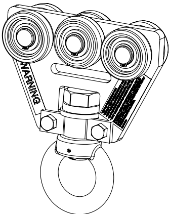
Diagram 6A. Tether Track® trolley installation.
