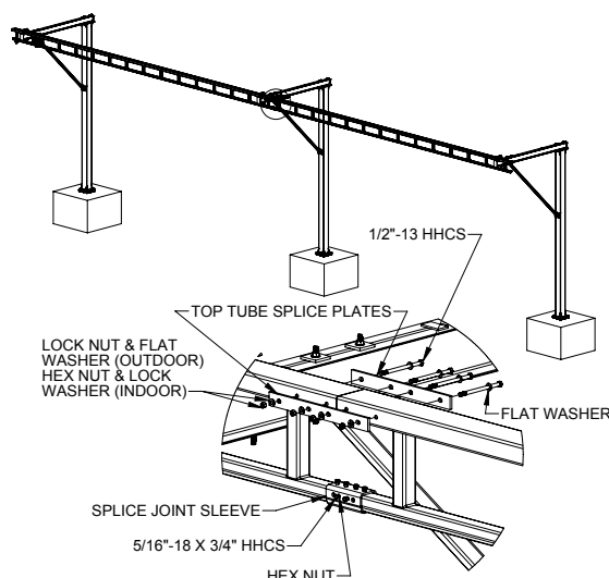
Diagram 5D. Sleeve style splice joint detail.
