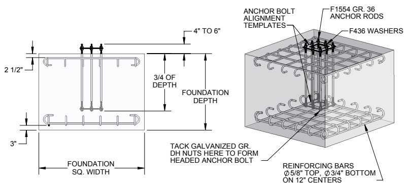
Diagram 2A. Cast-in Poured Foundation Detail.
