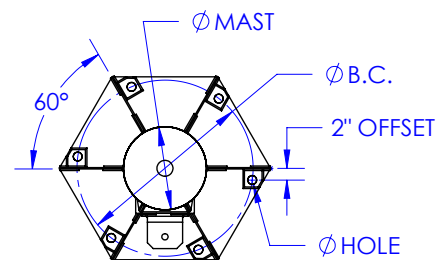
Diagram 3A. 6 bolt base bolt pattern.
