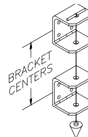
Diagram 2A. Plumbing formed channel brackets.
