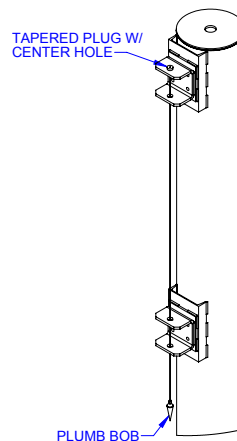
Diagram 3E. Plumbing the mast.
