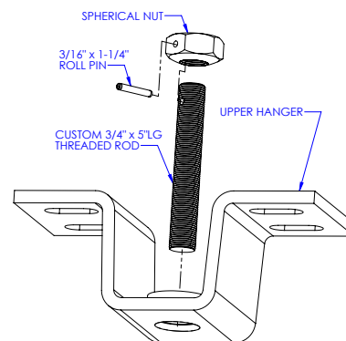
Diagram 5A. Assembling threaded rod to upper hanger.
