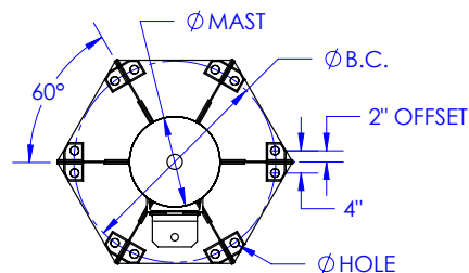
Diagram 3B. 12 bolt base bolt pattern.
