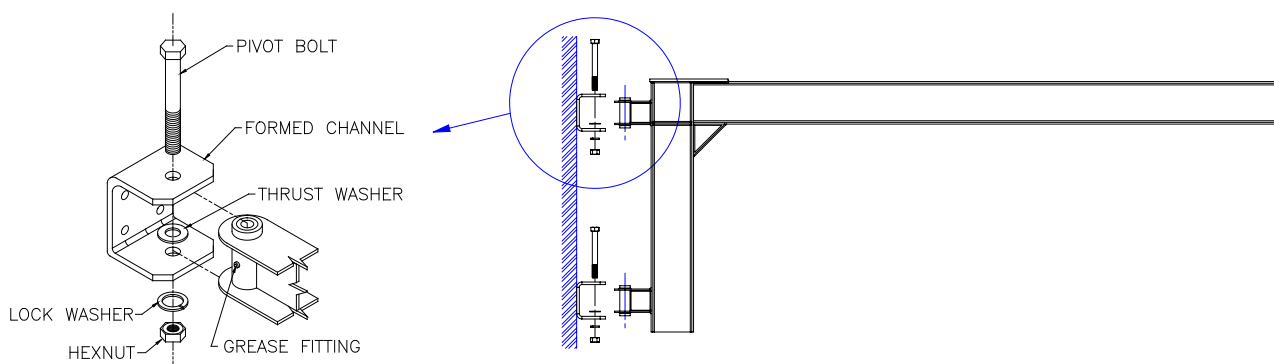
Diagram 2B. Attaching cantilever assembly to formed channel.
