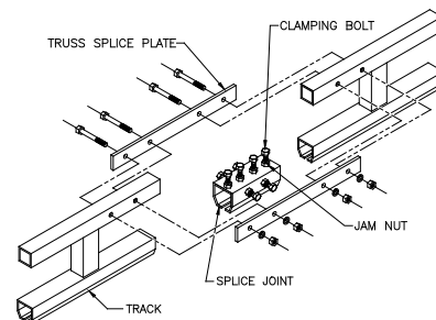
Diagram 5H. Splicing trussed track.
