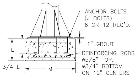
Diagram 3C. Poured foundation.
