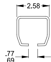
Diagram A. Track Opening Specification.
