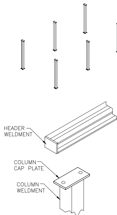
Diagram 2A. Orienting column cap plate.
