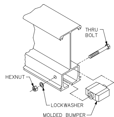
Diagram 5C. Installing end stop.
