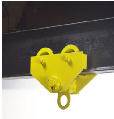
PLAIN TROLLEY
