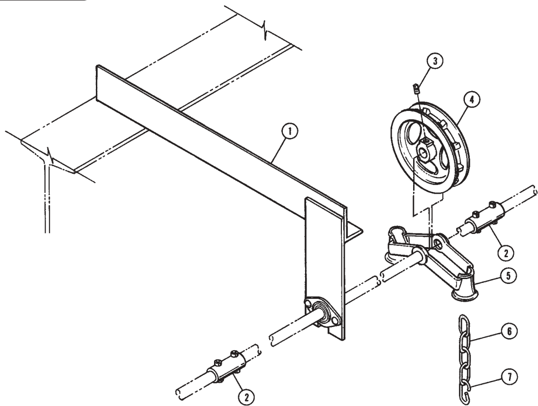
Figure 15. Hand Chain Drive. Catalog Numbers 904539 and 8282.
