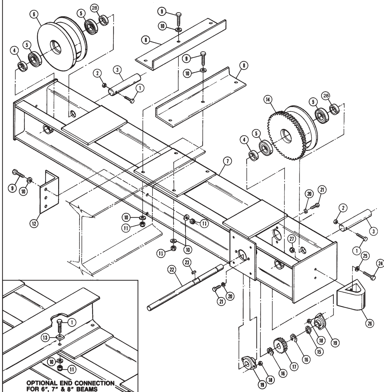
Figure 12. Geared Truck. Catalog Number 904536. (Only 1 Truck Shown) (Bumper is Optional. Catalog Number 904537.)
