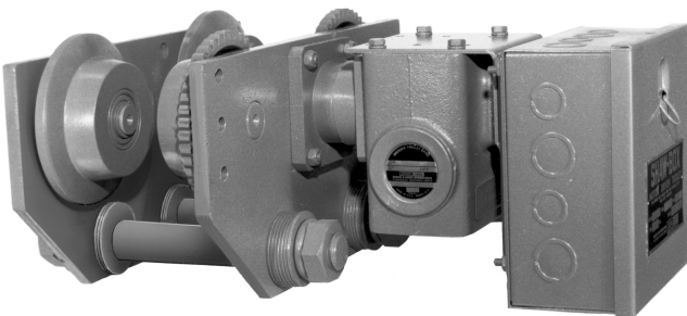
Figure 1. Standard Trolley
