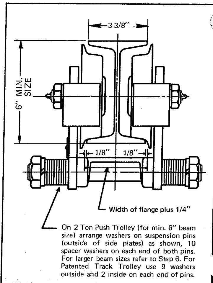
Figure 4. 2 Ton Push Trolley
