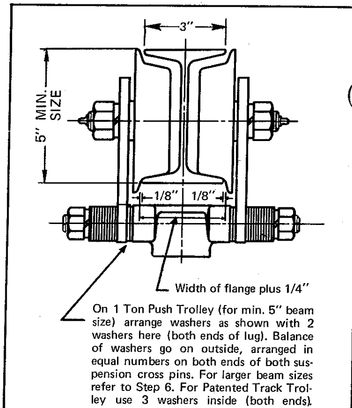
Figure 3. 1 Ton Push Trolley
