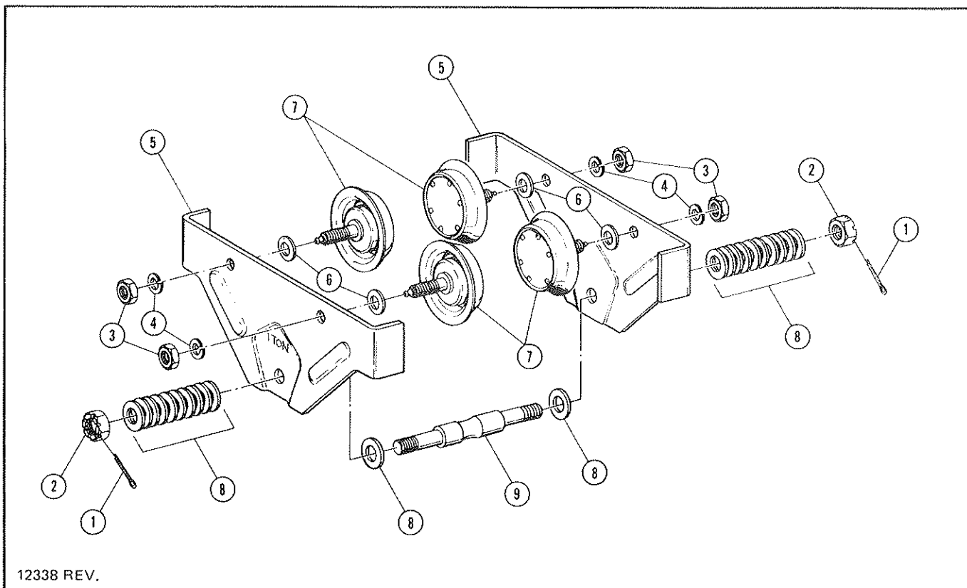
FIGURE 5. TRAILER (PLAIN) TROLLEY PARTS
