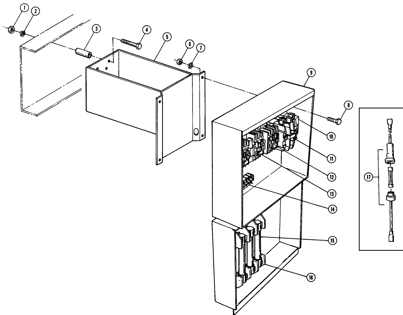
Figure 13. Electrical Enclosure and Mounting. Catalog Numbers 905385 thru 905387.
