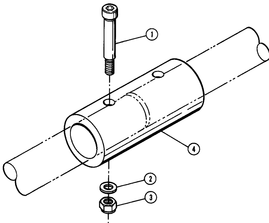
Figure 10. Coupling. Catalog Number 905374.
