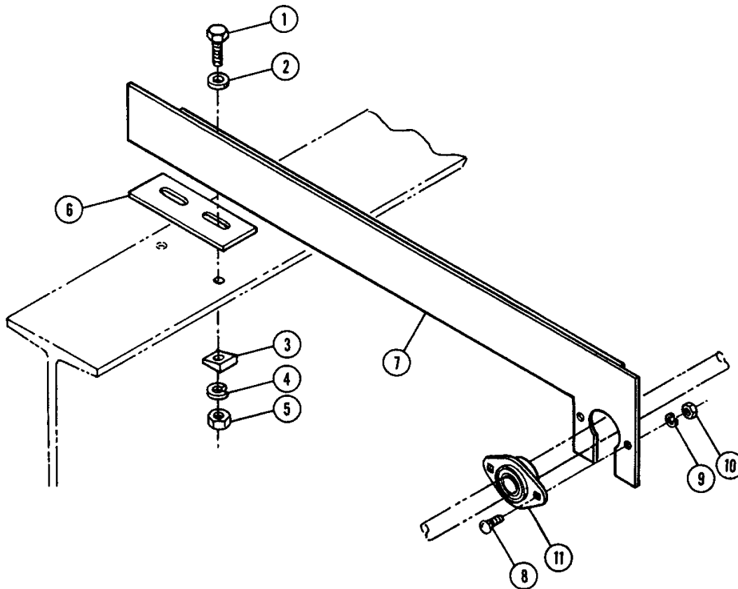
Figure 9. Cross Shaft Support. Catalog Number 905373.
