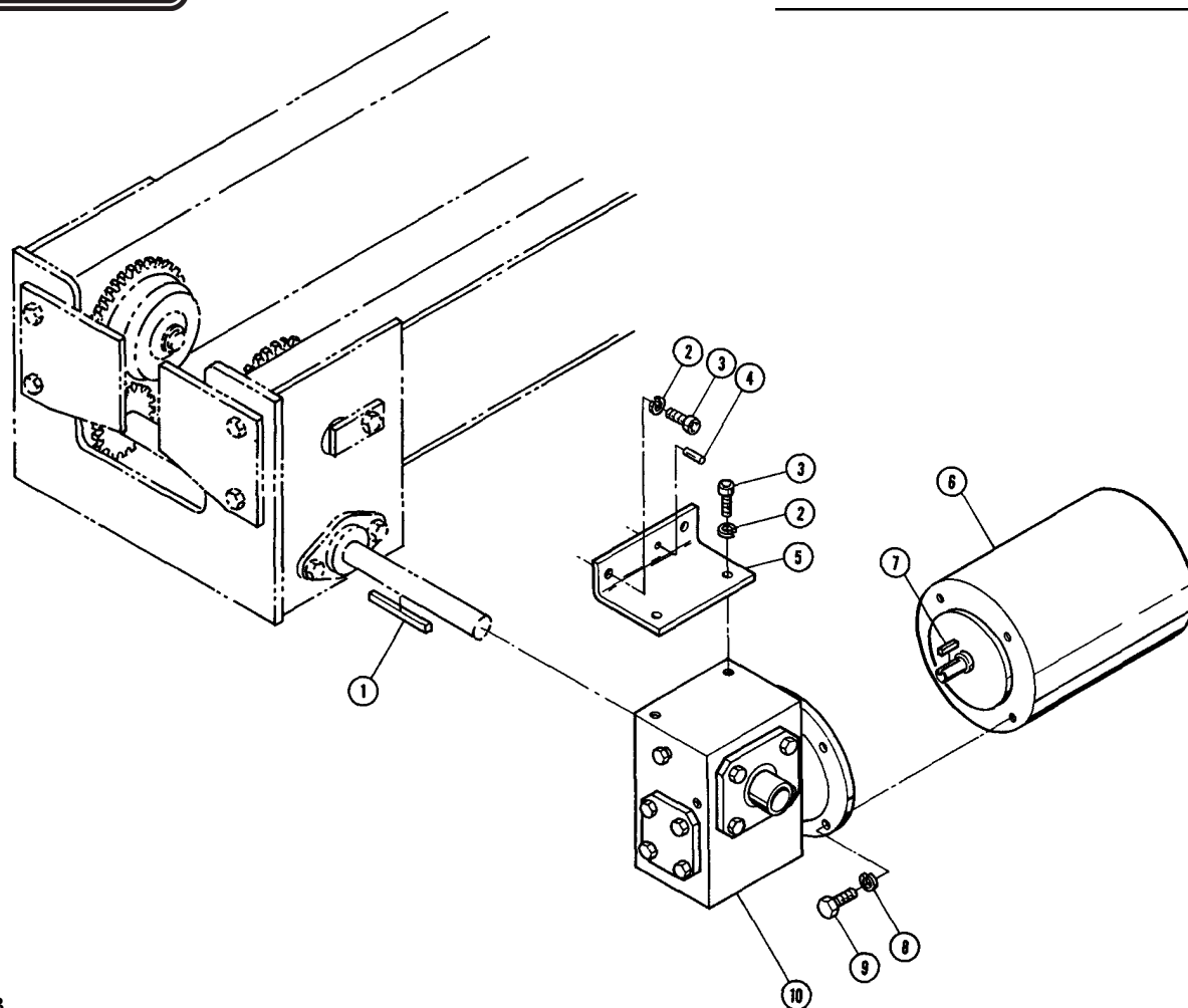
Figure 12. Gear Reducer. Catalog Numbers 905376 thru 905378) and motor (Catalog Numbers 905363, 905381, 905382 and 905394 thru 905396).
