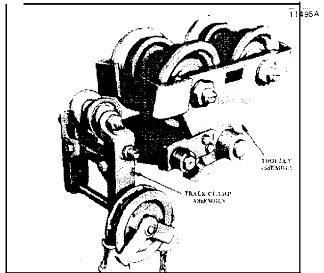
Figure 1-2. BUDGIT Track Clamp Shown Coupled To HI-GAP Trolley
