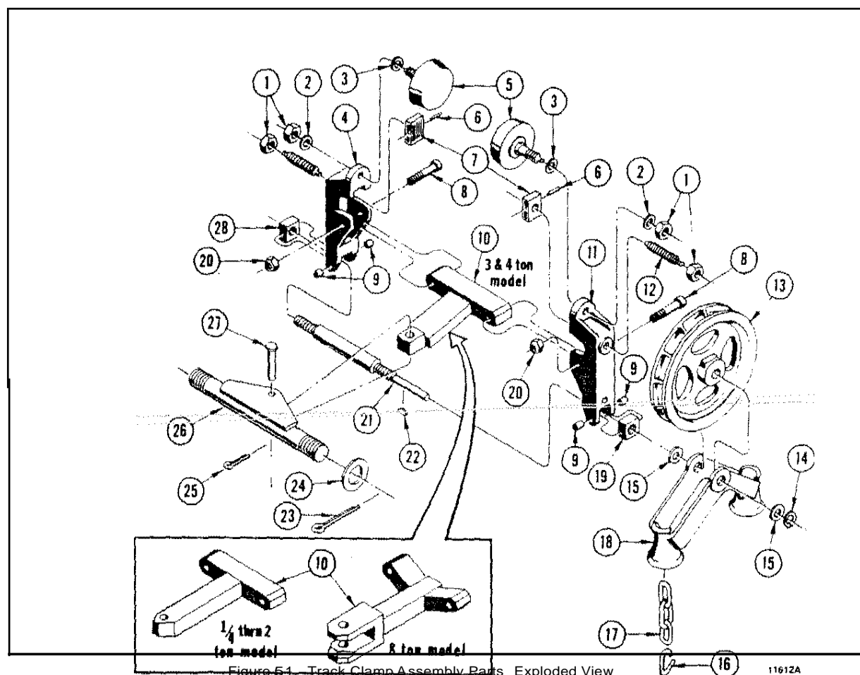
Figure 5-1. Track Clamp Assembly Parts Exploded View
