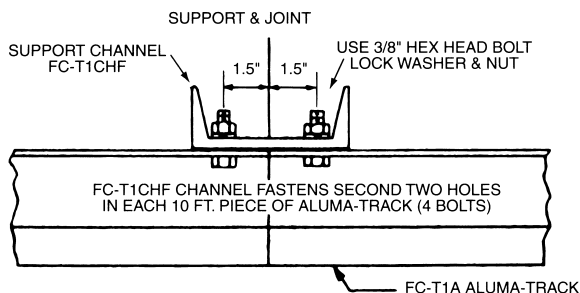
TRACK MOUNTING BRACKET 5\"/>
