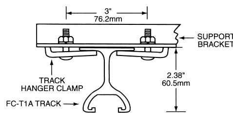
TRACK HANGER CLAMP (2 PIECE) FC-T1F
