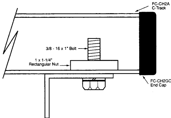
END STOP ASSEMBLY FC-CH2G
