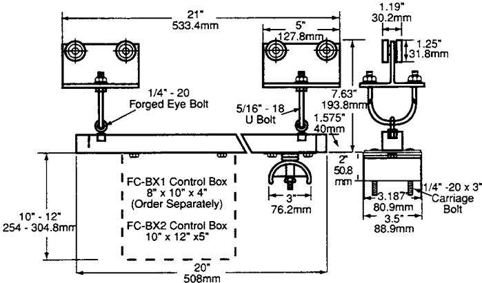
CONTROL TROLLEY ASSEMBLY FC-TRC22
