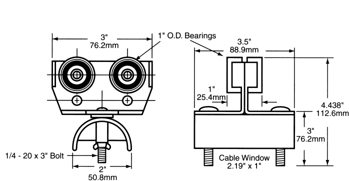
TROLLEY ASSEMBLY FC-TR2
