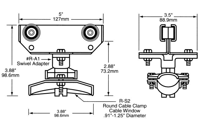
TROLLEY ASSEMBLY R-TR1B
