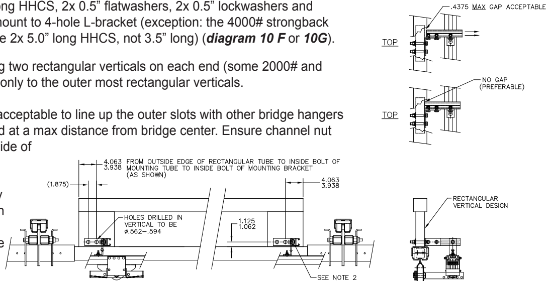
Diagram 10F. Steel bridge with rectangular vertical.
