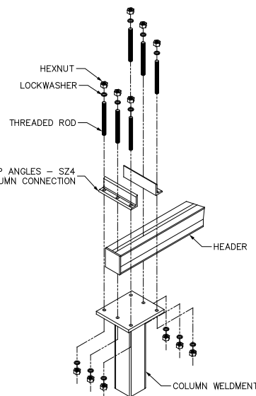
Diagram 3C. Installing header weldments on 6-bolt column cap plates.
