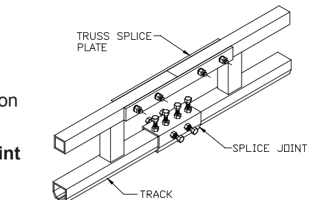
Diagram 4E. Spliced tracks.
