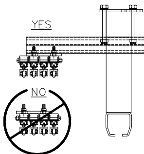
Diagram 10S. Conductix installation orientation.
