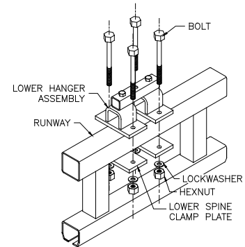
Trussed Track 4000#
