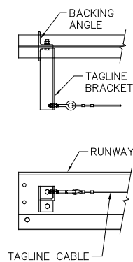
Diagram 9G. Tagline on aluminum runway.
