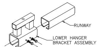
Plain Track 4000#
