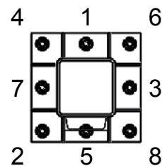
Diagram 2D. Anchor nut tightening pattern.
