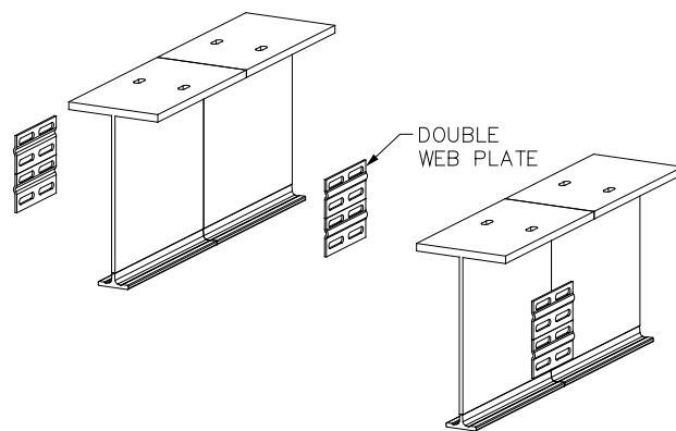
Diagram 3D. Welded splice (5000 & Larger Tarca® beam).
