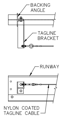
Diagram 9C. Tagline on aluminum runway.
