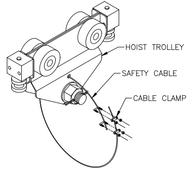
Diagram 6F. Installing safety cable on hoist trolley.
