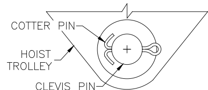
Diagram 6K. Installing cotter pin through trolley clevis pin.
