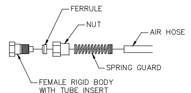
Diagram 10D. Female fitting assembly.
