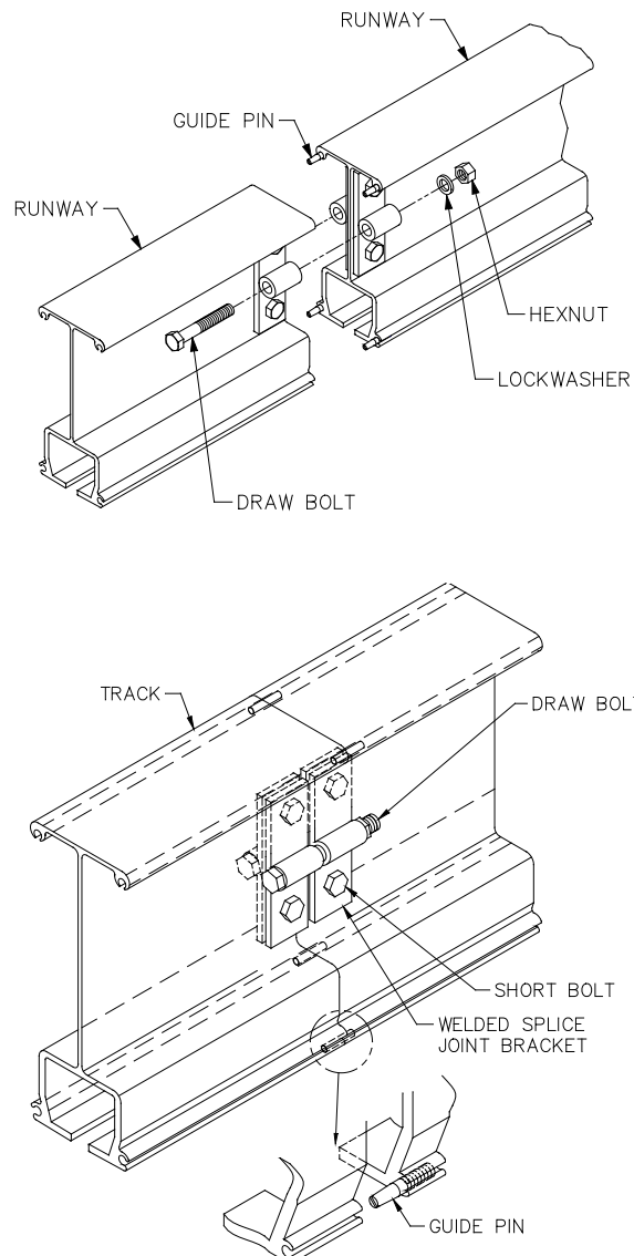
Diagram 4A. Splicing Aluminum track sections.
