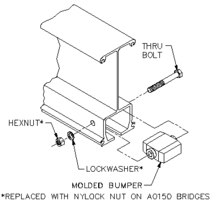
Diagram 3C. Installing standard endstop.
