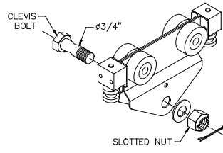
Diagram 6H. Installing hoist on A250-A500 hoist trolley.
