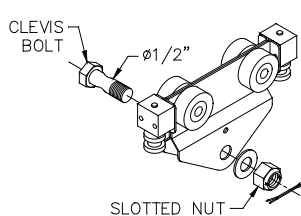
Diagram 6G. Installing hoist on A150 hoist trolley.
