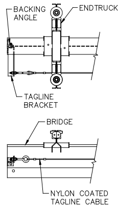
Diagram 9B. Tagline on non-coped aluminum bridge.
