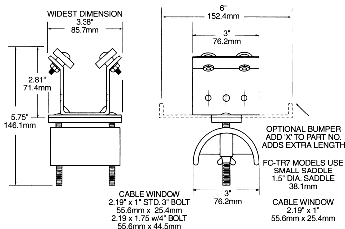
TROLLEY ASSEMBLY FC-TR6
