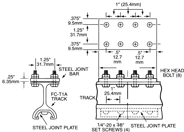
TRACK JOINT KIT (2 PIECE) BAR & PLATE FC-T1D
