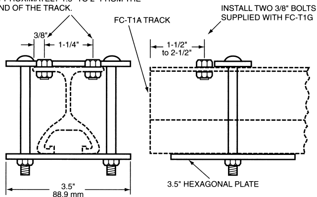
END STOP FC-T1G
