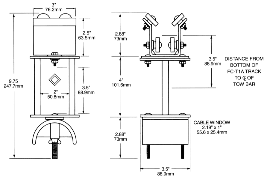
TOW TROLLEY ASSEMBLY FC-TRT6Z
