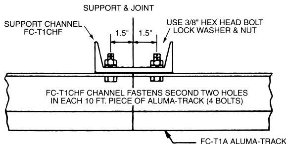
TRACK MOUNTING BRACKET 5\"/>
