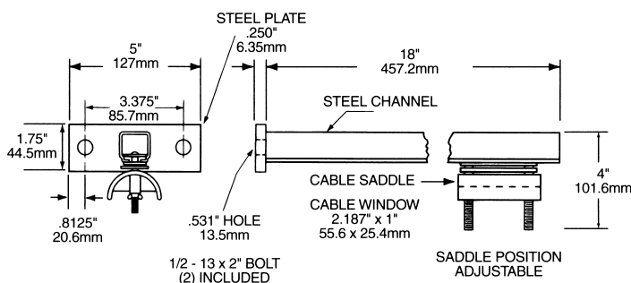
TOW ARM ASSEMBLY FC-TB4
