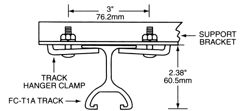
TRACK HANGER CLAMP (2 PIECE) FC-T1F
