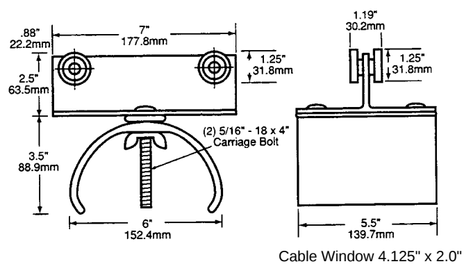
TROLLEY ASSEMBLY FC-TR24
