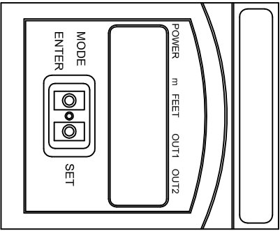
PHOTO-EYE SENSOR TOP VIEW
