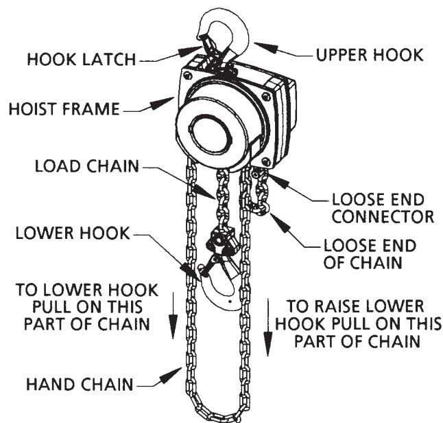
Figure 2 – Main Parts of Hurricane 360 Hoist
