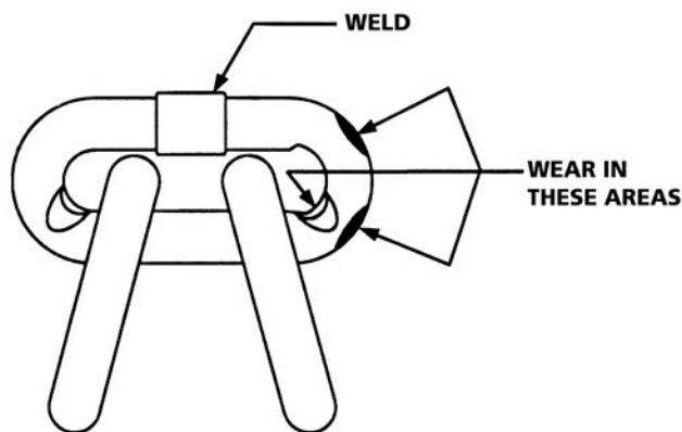
Figure 4 - Chain Inspection
