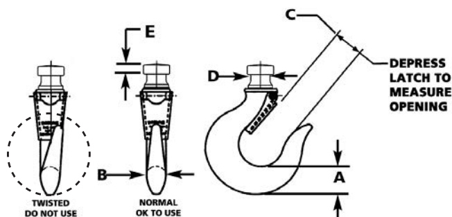
Figure 3 - Hook Inspection
